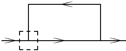
FIG. 1: In the path integral one can take all paths (a) that go forward in time, but one excludes all paths (b) that go backward in time.
