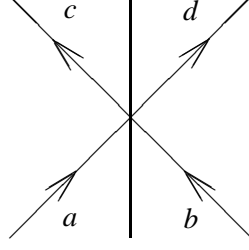
FIG. 4: The beam splitter transmits with an amplitude \alpha and reflects with an amplitude i\beta . The factor of i preserves unitarity.
