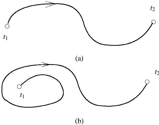
FIG. 1: In the path integral one can take all paths (a) that go forward in time, but one excludes all paths (b) that go backward in time.
